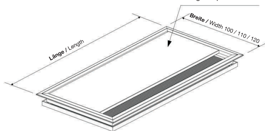
Gerader Klappdeckel / Straight flap Cover
